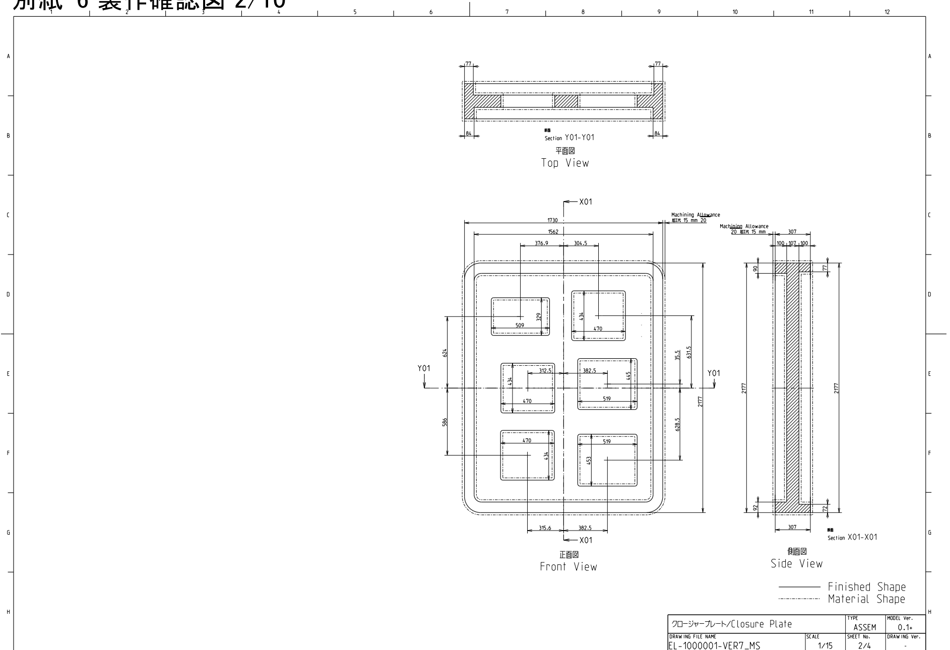
図2 Closure Plate
