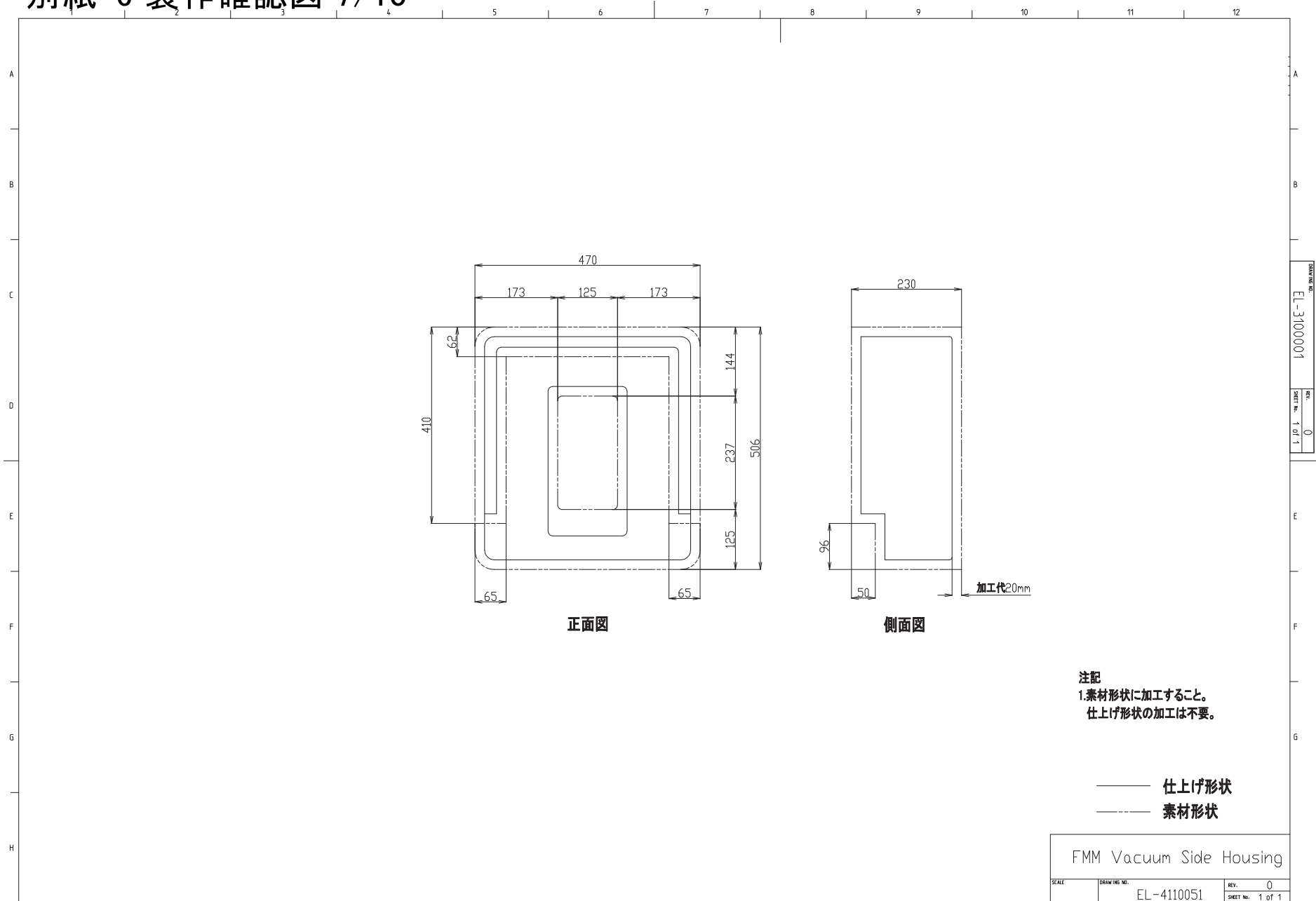
図7 Fixed Mirror Module Vacuum-Side Housing
