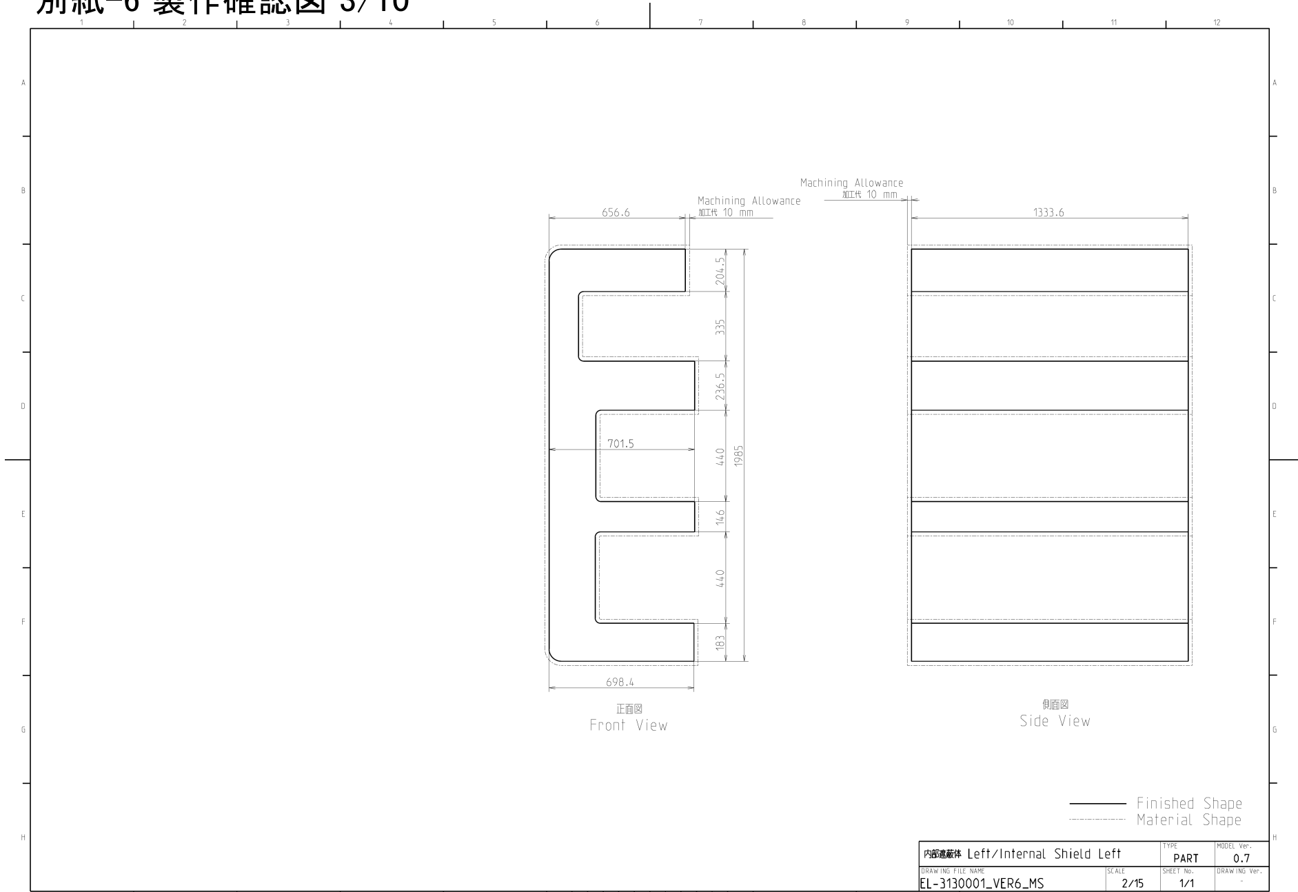
図3 Internal Shield Left
