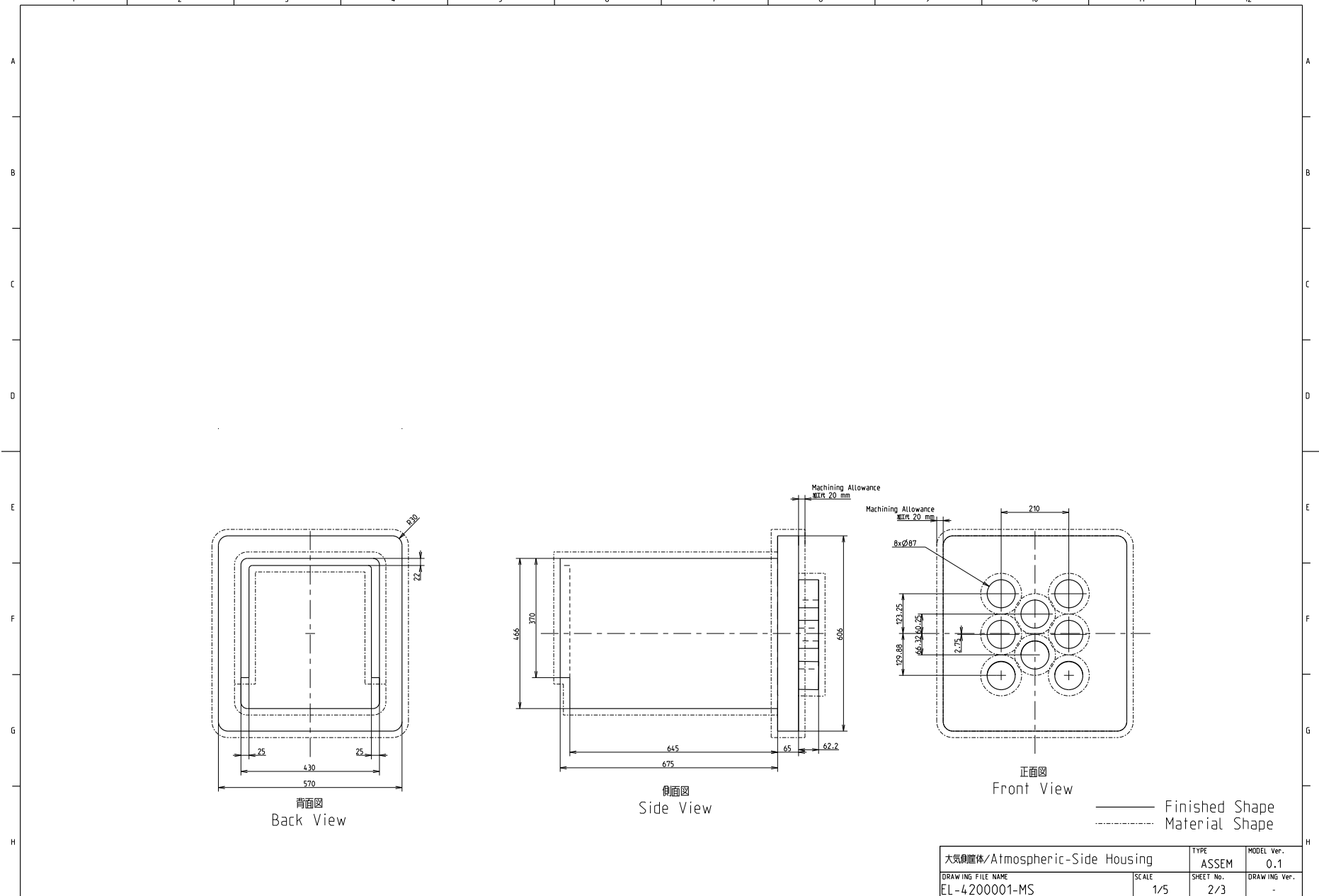
図6 Fixed Mirror Module Atmospheric-Side Housing
