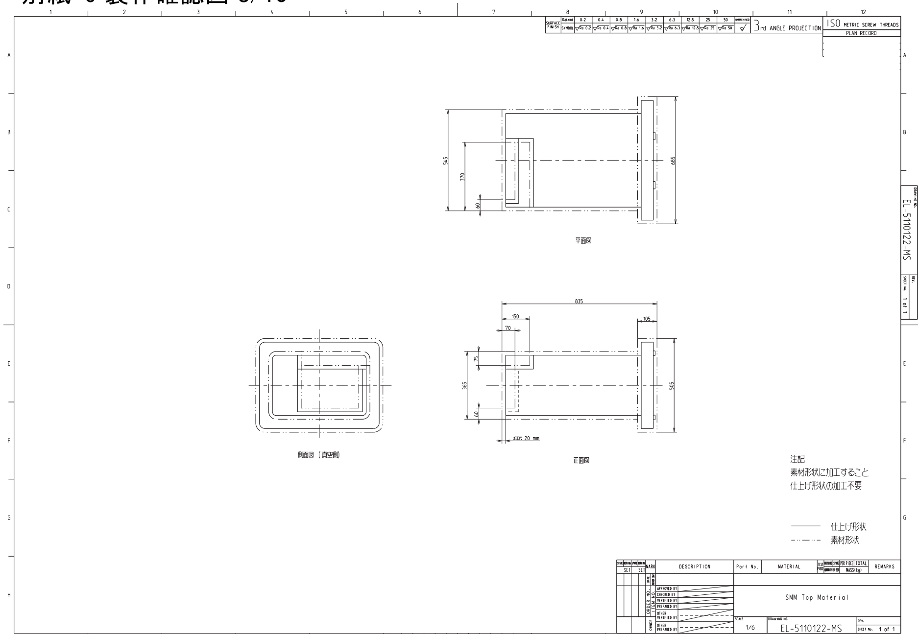
図8 Steering Mirror Module Housing (Top)
