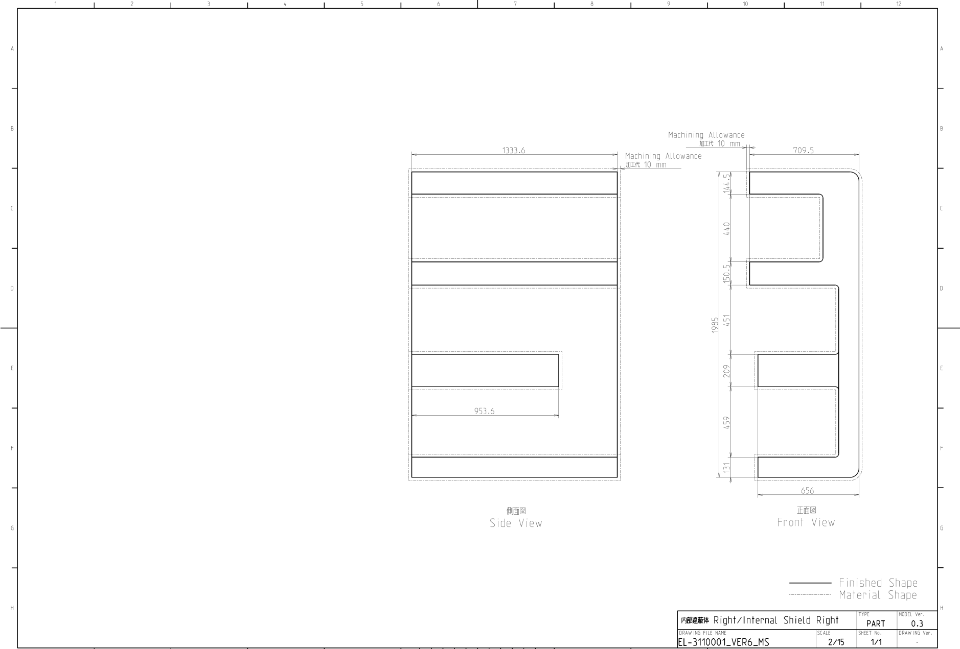
図4 Internal Shield Right
