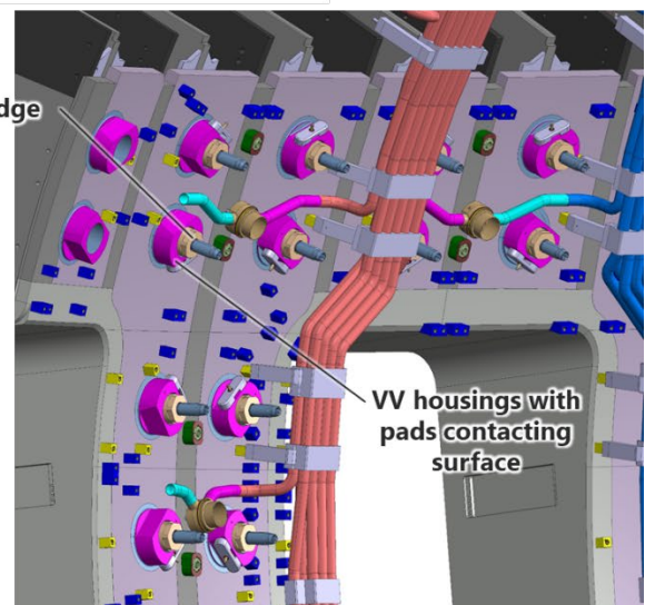
(b) Outboard
