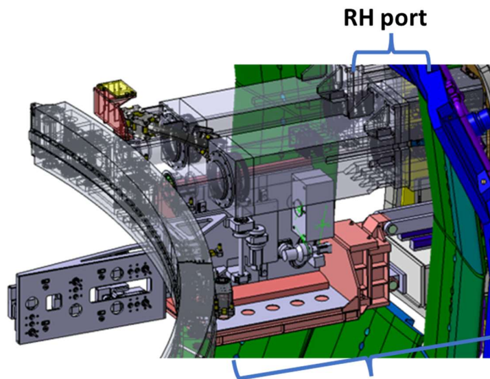
IPT deploying NBDL-RH tool with MTPP
