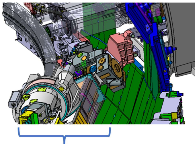
VMNP gripping NBDL-RH tool on MTPP
