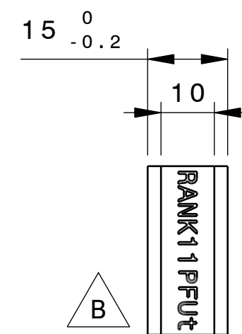
AUXILIARY VIEW H Scale: 1:1
