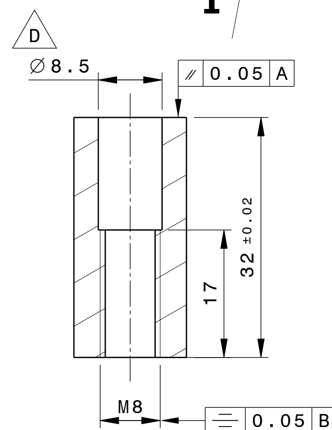
SECTION VIEW G-G
