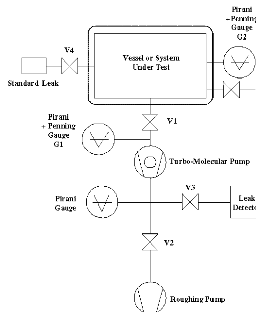
Figure 12-1 Typical Leak Detection Equipment/ 典型的なリーク検知装置
