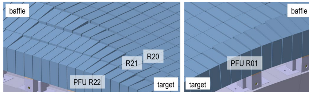
Fig. 4.3-1: Illustration of the transition area between target and baffle at downstream side (R20, R21, R22) and upstream side (R01).
