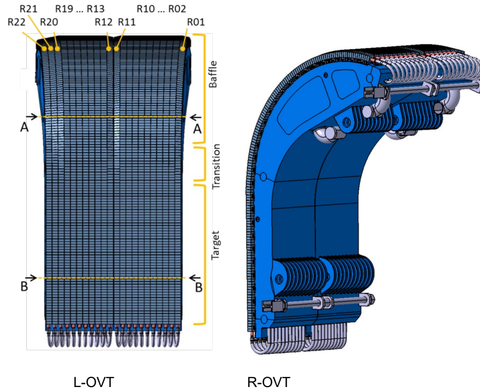
Figure 4.1-1: schematic 3D illustration of the standard OVT. PFU R1 is located at the upstream side of OVT and PFU R22 is at the downstream side. Cooling water in PFU flows from straight part (high heat flux handling part) to baffle part.
