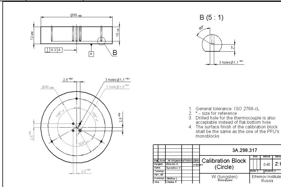
Figure 4.11-1: possible geometry of calibration block for infrared measurements
