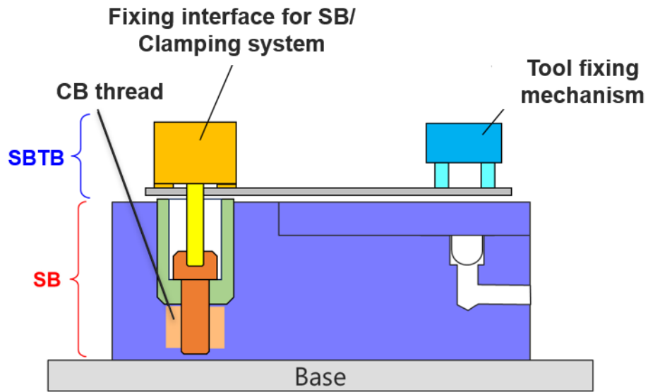
(a) SBTB installation
