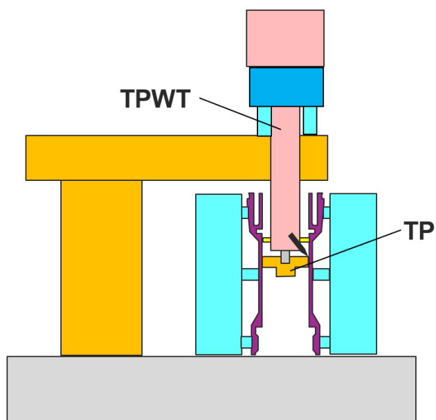
(b)TPWT installation · TP welding
