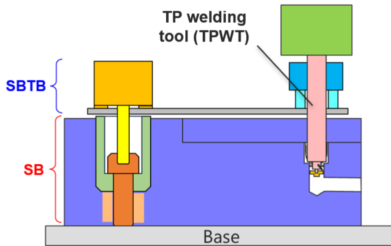
(b) TPWT installation – TP welding
