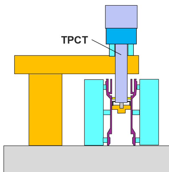
(c)TPCT installation · TP cutting
