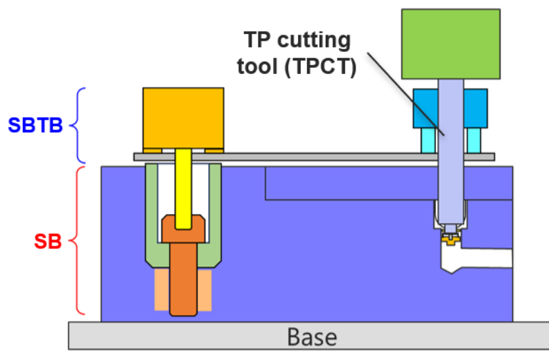
(c) TPCT installation – TP cutting
